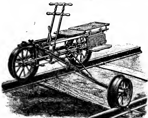
Fig. 5607. SHEFFIELD VELOCIPEDE-CAR No. 2. For Rider and Passenger. Weight, 140 lbs.
